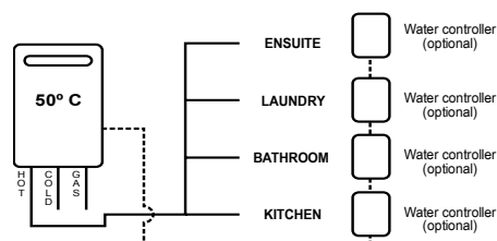
Diagram 1 - 50°C Appliance
